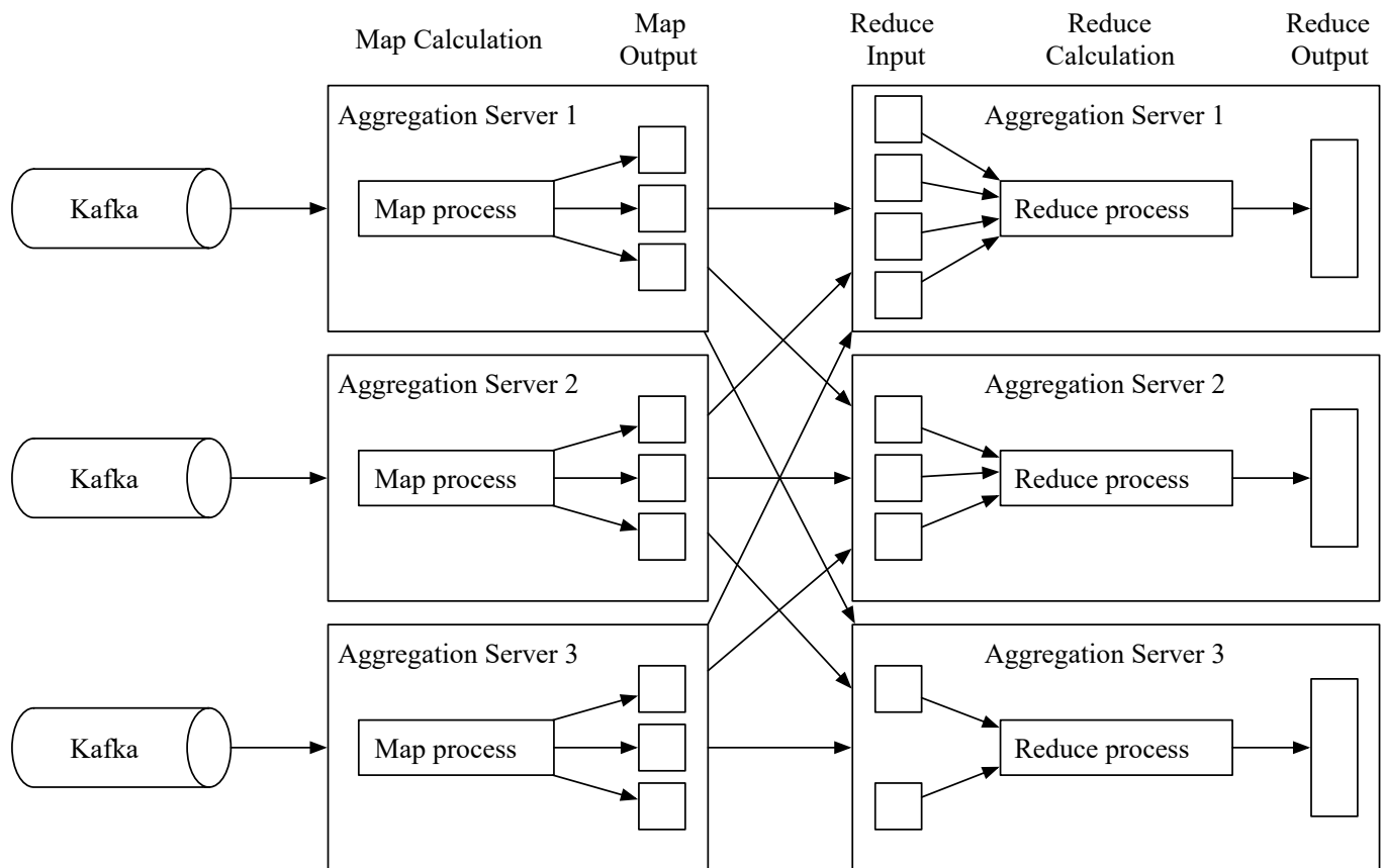
Figure 22 Aggregation service
