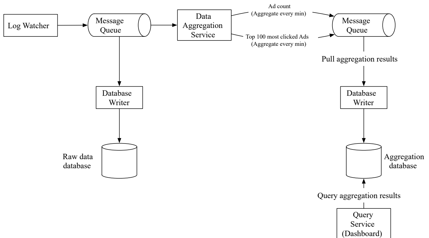
Figure 3 High-level design
