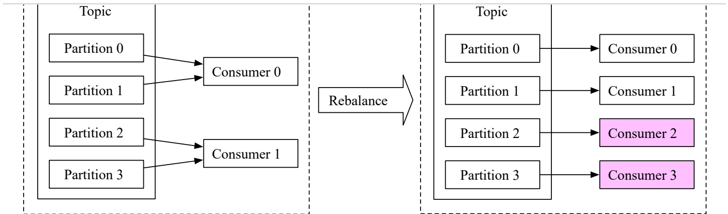
Figure 21 Add consumers
