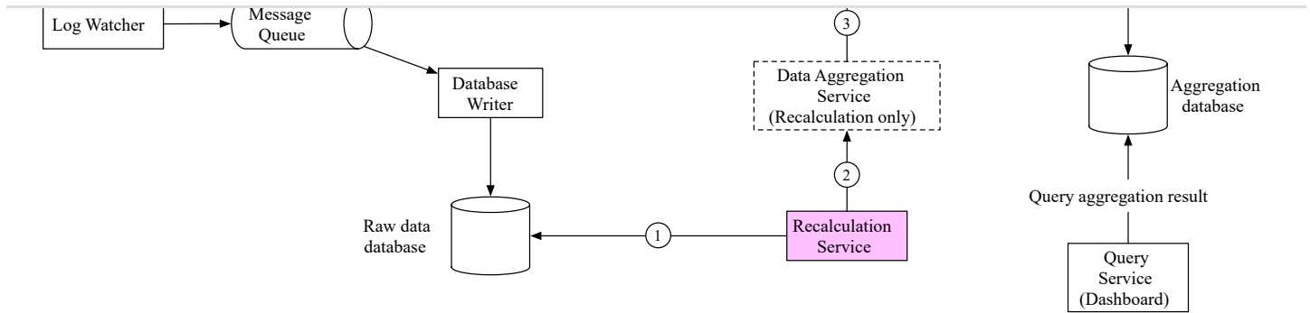
Figure 11 Recalculation service
