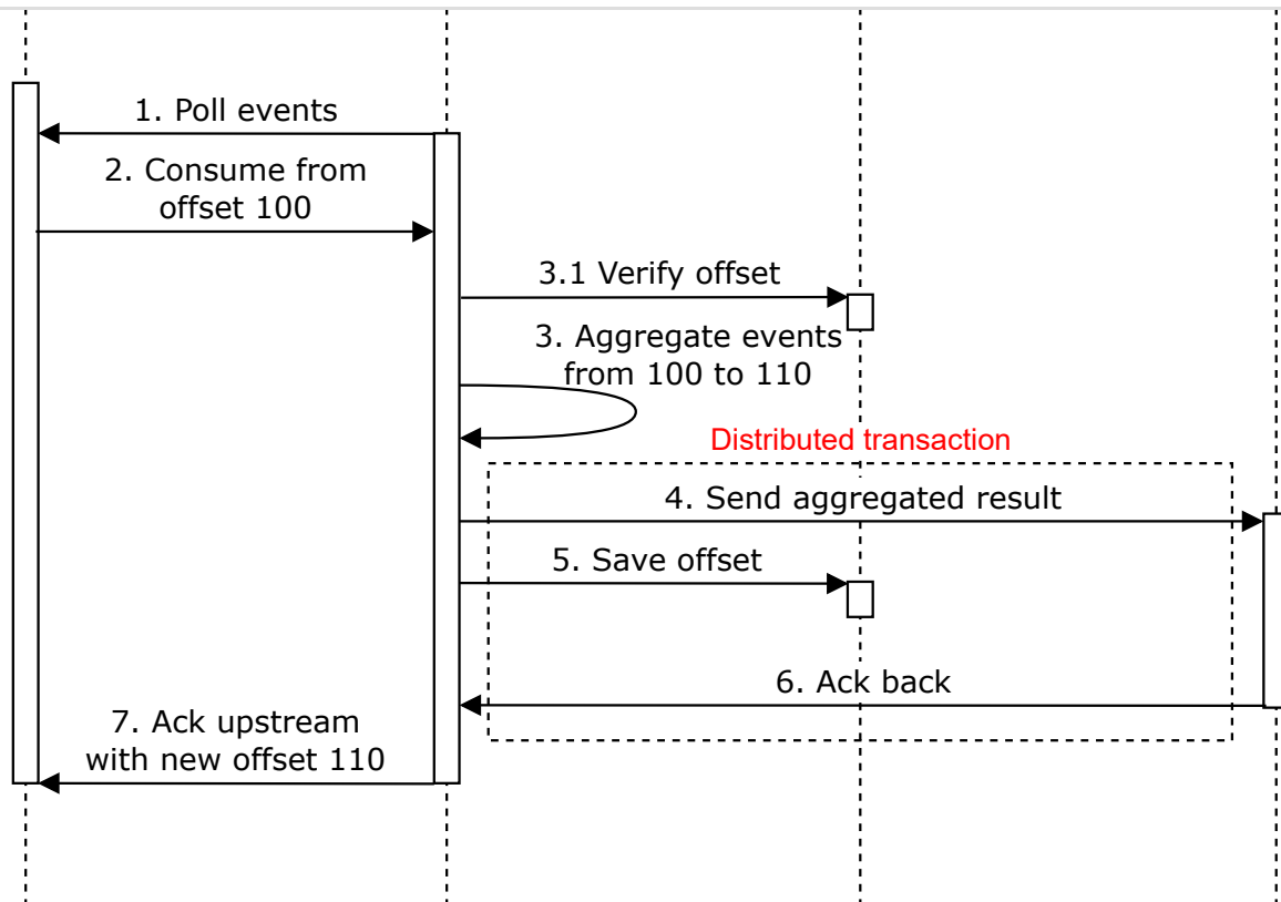
Figure 20 Distributed transaction
