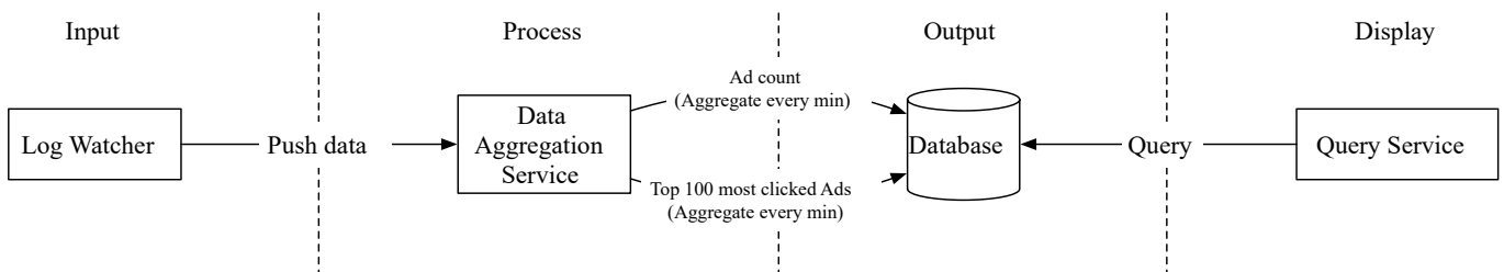
Figure 2 Aggregation workflow
