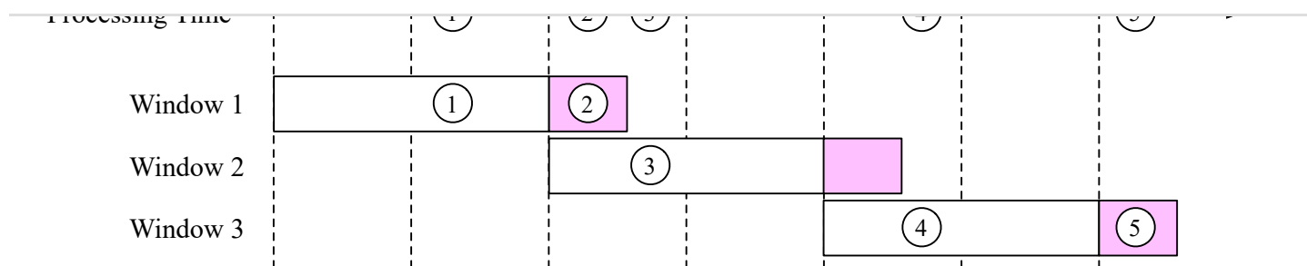
Figure 14 Watermark
