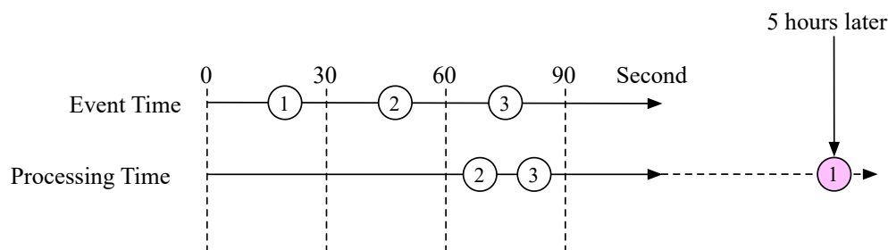
Figure 12 Late events
