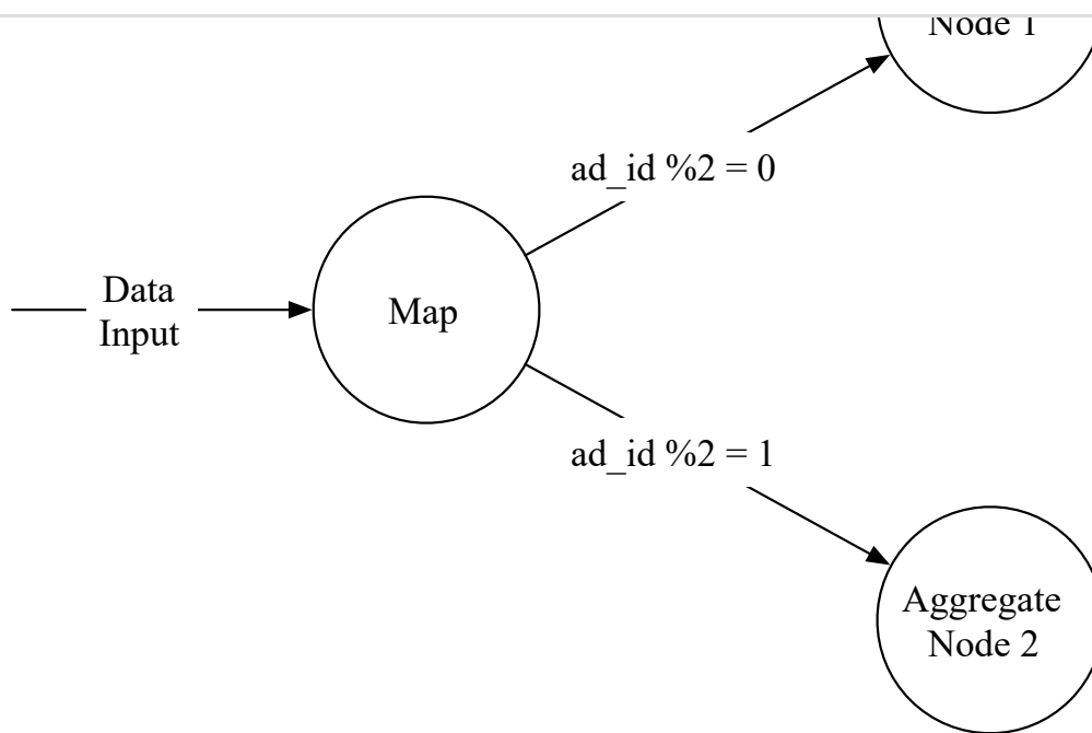
Figure 6 Map operation
