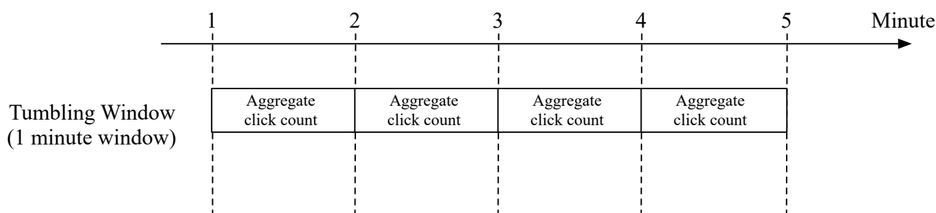
Figure 15 Tumbling window
