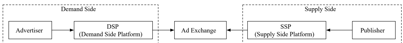
Figure 1 RTB process
