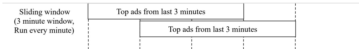
Figure 16 Sliding window
