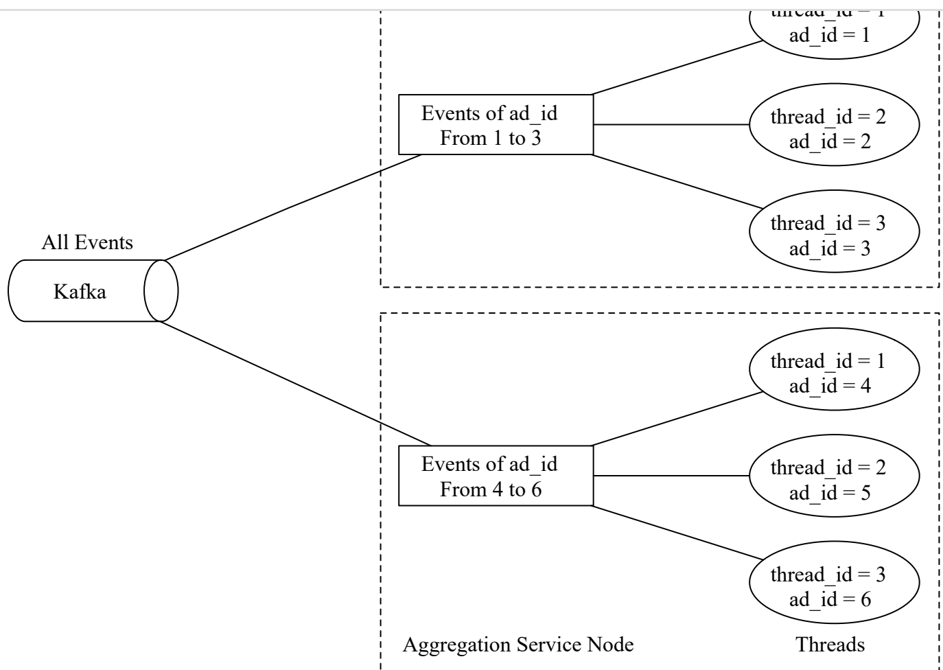
Figure 23 Multi-threading
