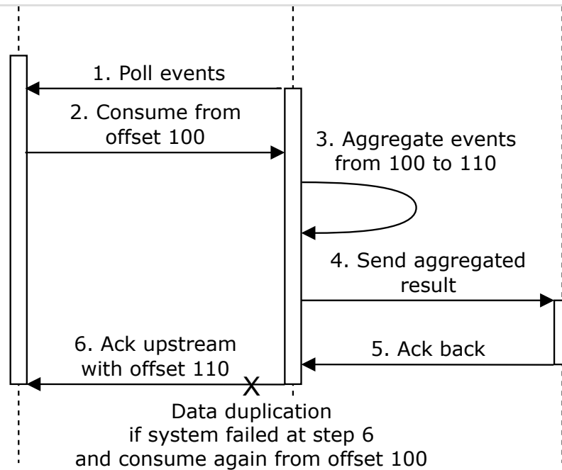
Figure 17 Duplicate data
