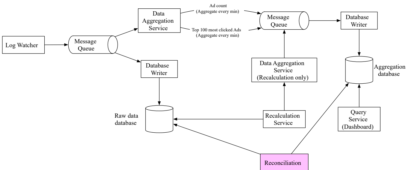
Figure 28 Final design
