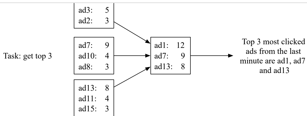
Figure 7 Reduce node
