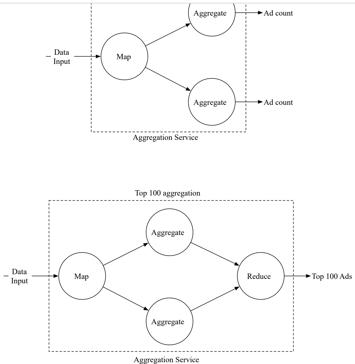
Figure 5 Aggregation service
